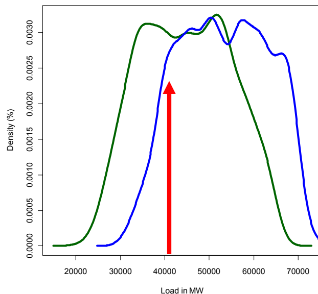
Figure 7: Kernel density estimation of load (blue line) and residual load (green line) (10/2008 – 11/2009)
