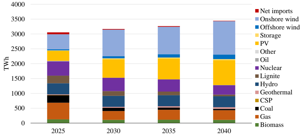
Figure 2: EU electricity generation in the REF scenario
