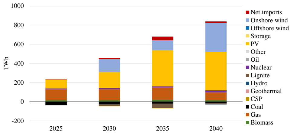
Figure 3: Additional electricity generation in the EUQ scenario
